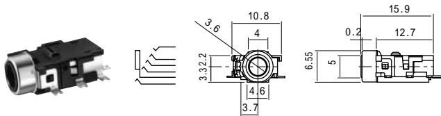
No.M03-809A0 (3.5 -6極) SMT 6-CONDUCTOR MINIATURE JACK FOR P.C.B.
