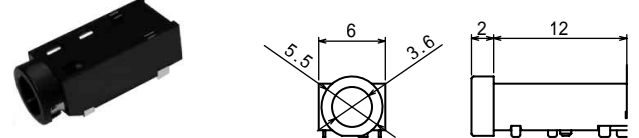
No.MJ-3935-4 (3.5 -4極) SMT 4-CONDUCTOR MINIATURE JACK FOR P.C.B
