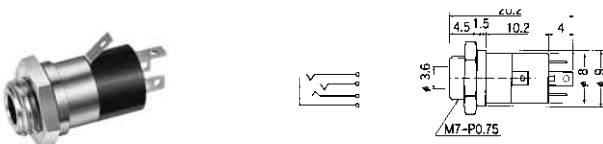
No.MJ-064H (3.5 -4極) PANEL MOUNT MINIATURE JACK
