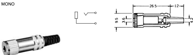
No.MJ-166M (3.5 -2極) MINIATURE INLINE JACK MONO
