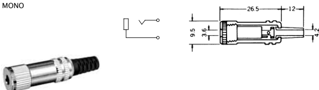
No.MJ-166M (3.5 -2極) MINIATURE INLINE JACK MONO
