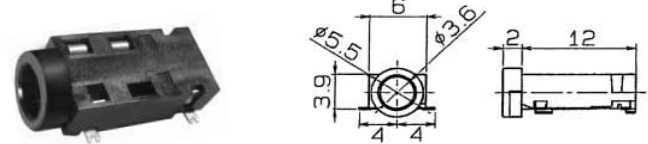
No.MJ-064SP (3.5 -4極) SNAP-IN MOUNT MINIATURE JACK
