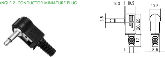
No.MP-105L (3.5 -2極) 2-CONDUCTOR MINIATURE PLUG. MONO
