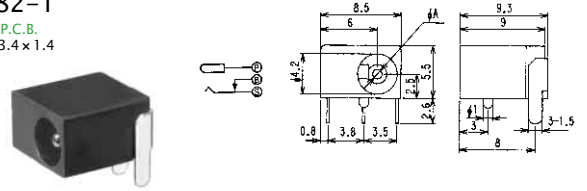
No.MJ-84 DC JACK FOR P.C.B. PLUG TYPE: 3.4 × 1.4 (DC6V 0.5A)
