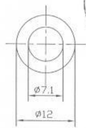
WASHER 1 PC t=0.4
